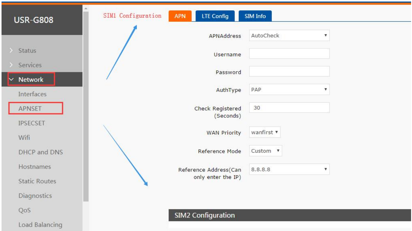
Diagram 3.2.9-1 APN configuration
