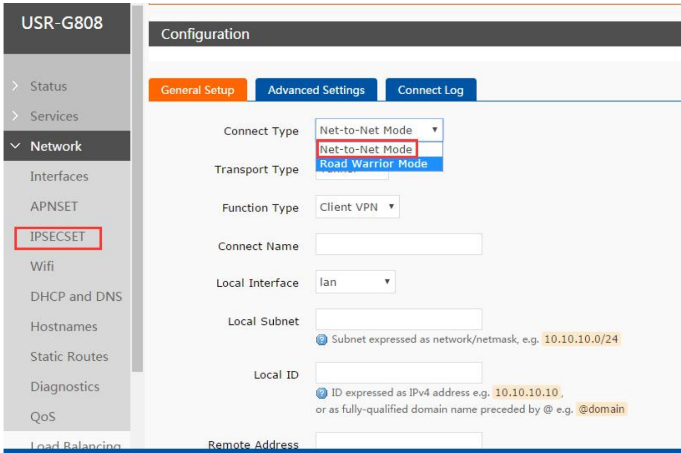
Diagram 3.2.12.3-1 IPSEC Configuration
