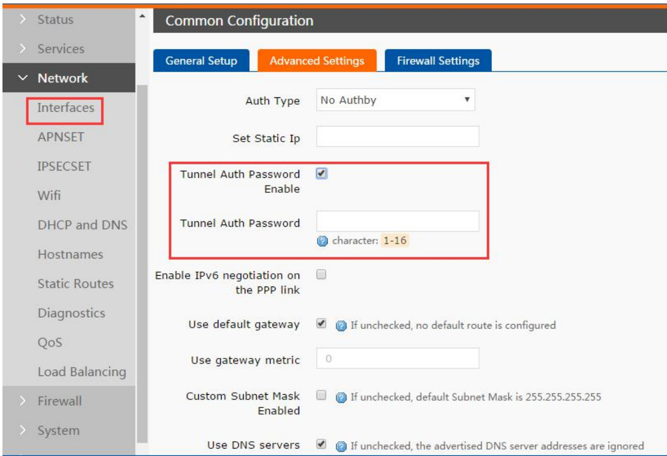
Diagram 3.2.12.2-2 L2TP Client configuration 2
