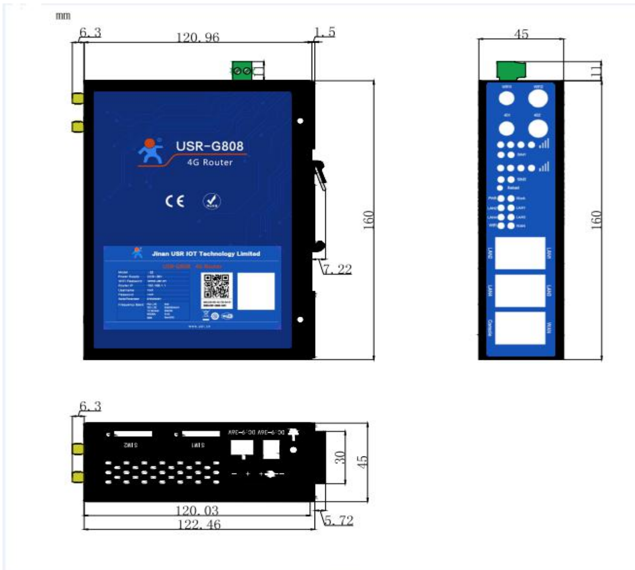
Diagram 2.4-2 Dimension
